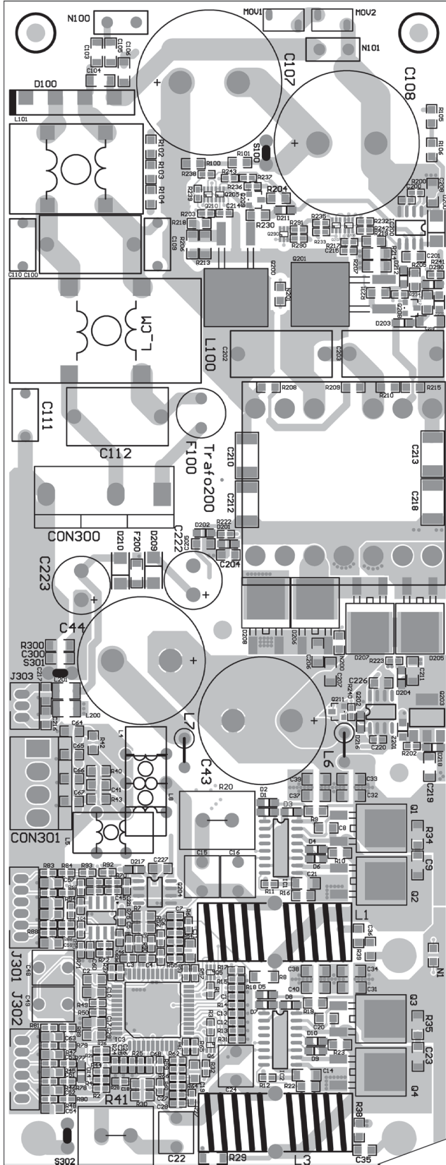
Figure 3. Amplifier/SMPS PCB (Non-RoHS) Topside Etch Layout
