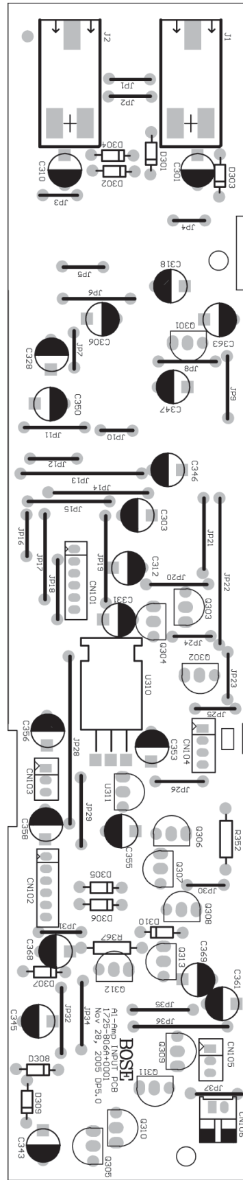
Figure 14. Input/Limiter PCB (RoHS) Bottom Side Etch Layout
