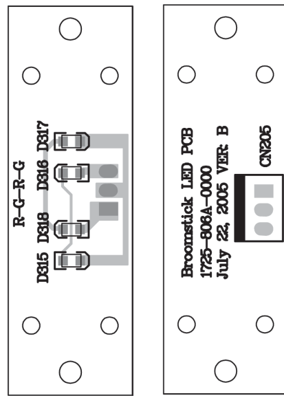
Figure 16. Signal/Overload LED PCB Etch Layout
