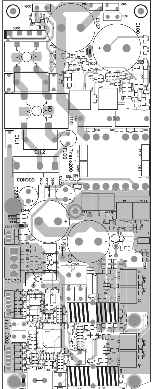
Figure 4. Amplifier/SMPS PCB (Non-RoHS) Internal Etch Layer 1 Layout
