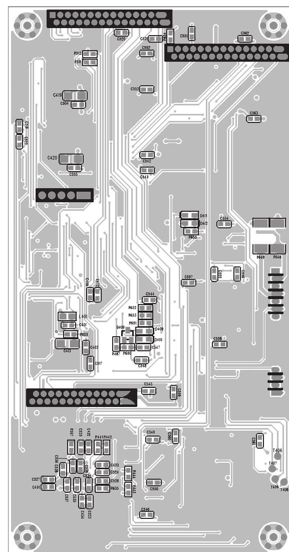
BOTTOM SILKSCREEN AND ETCH
