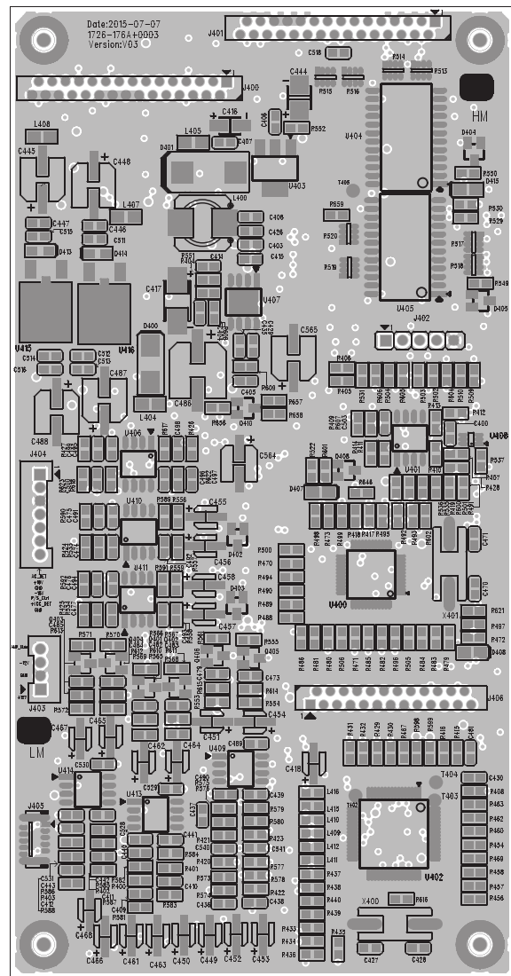
TOP SILKSCREEN AND GND ETCH
