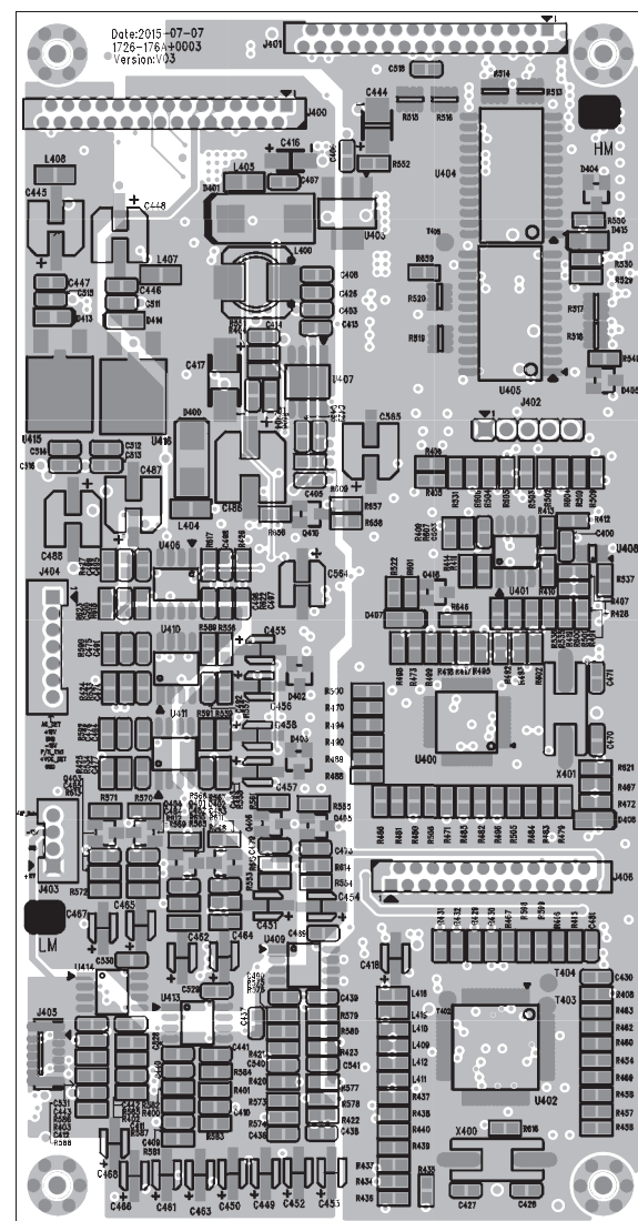
TOP SILKSCREEN AND POWER ETCH
