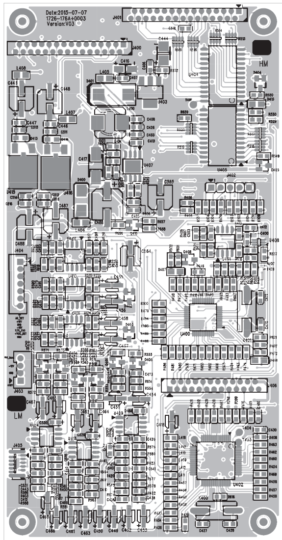
TOP SILKSCREEN AND ETCH
