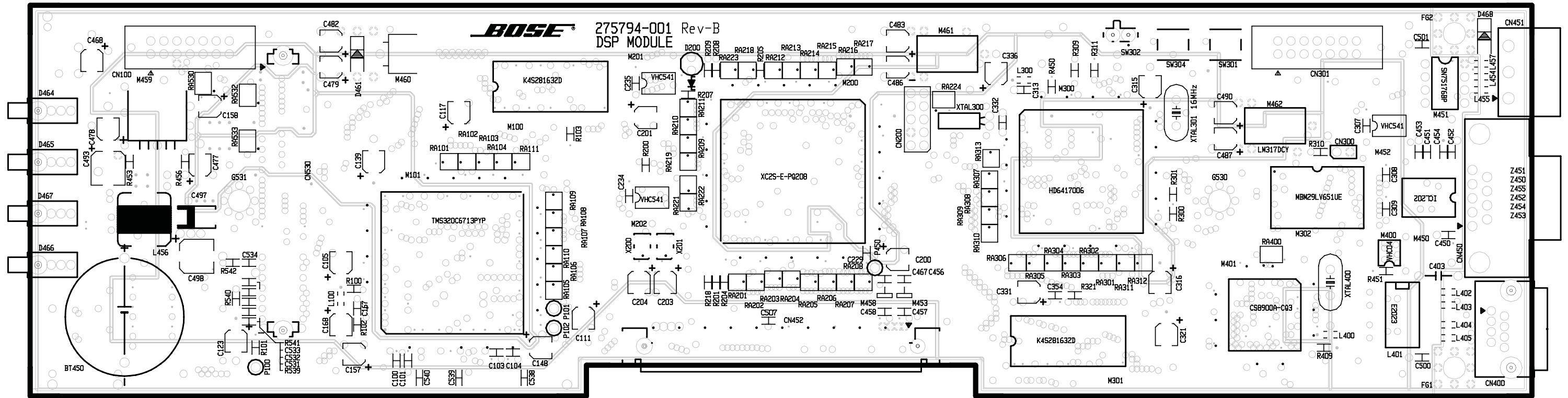
DSP PCB L3 GND Etch Layout Diagram
