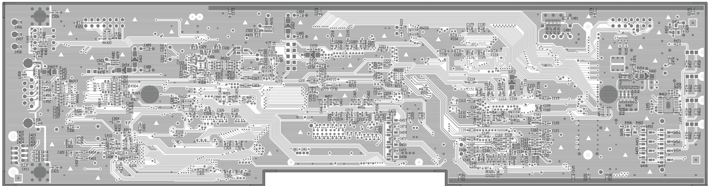
DSP PCB L4 Bottom Etch Layout Diagram ControlSpace® ESP-88C and ESP-00 Chassis
