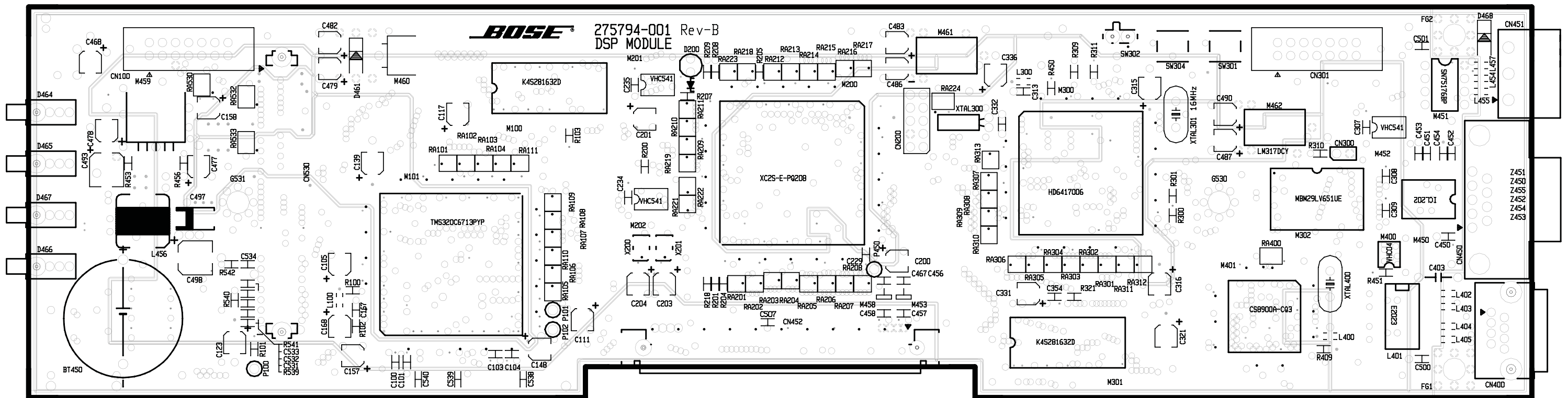
DSP PCB L2 VCC Etch Layout Diagram ControlSpace® ESP-88C and ESP-00 Chassis
