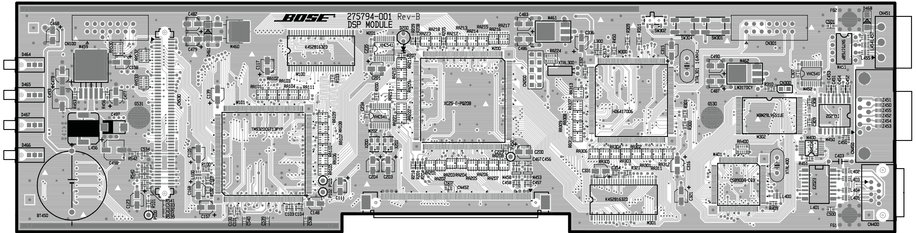
DSP PCB L1 Topside Etch Layout Diagram
