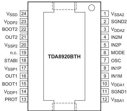
Pin Configuration
