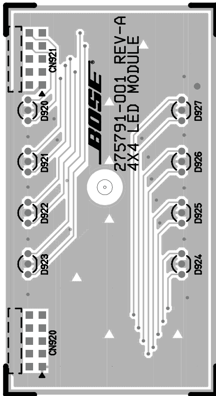
LED PCB Topside Etch Layout Diagram
