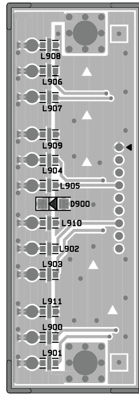
Output PCB Bottom Etch Layout Diagram
