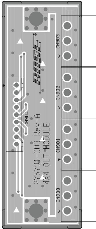
Output PCB Topside Etch Layout Diagram
