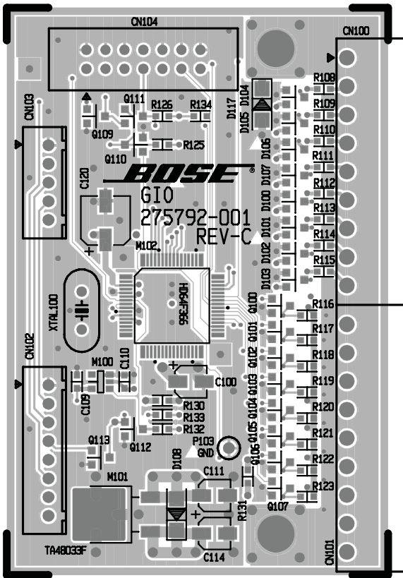
GPIO PCB Topside Etch Layout Diagram
