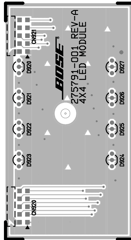
LED PCB Bottom Etch Layout Diagram
