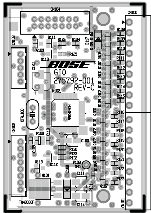
GPIO PCB VCC Etch Layout Diagram
