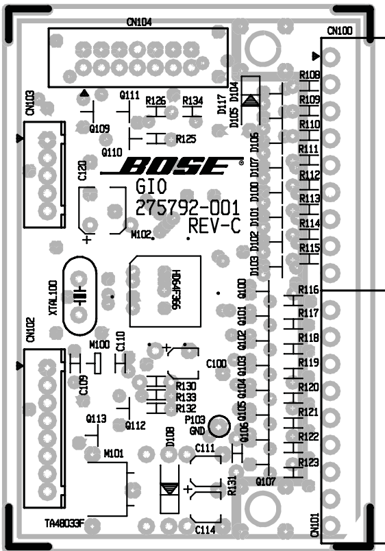
GPIO PCB GND Etch Layout Diagram
