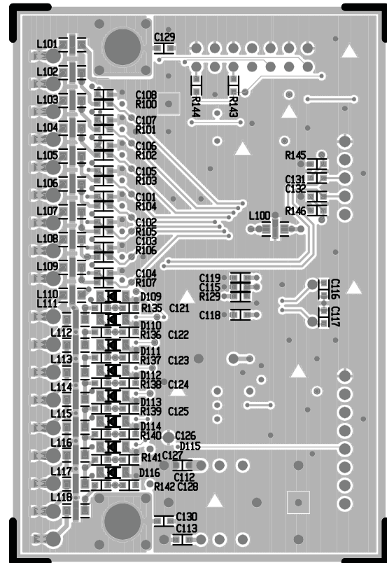
GPIO PCB Bottom Etch Layout Diagram
