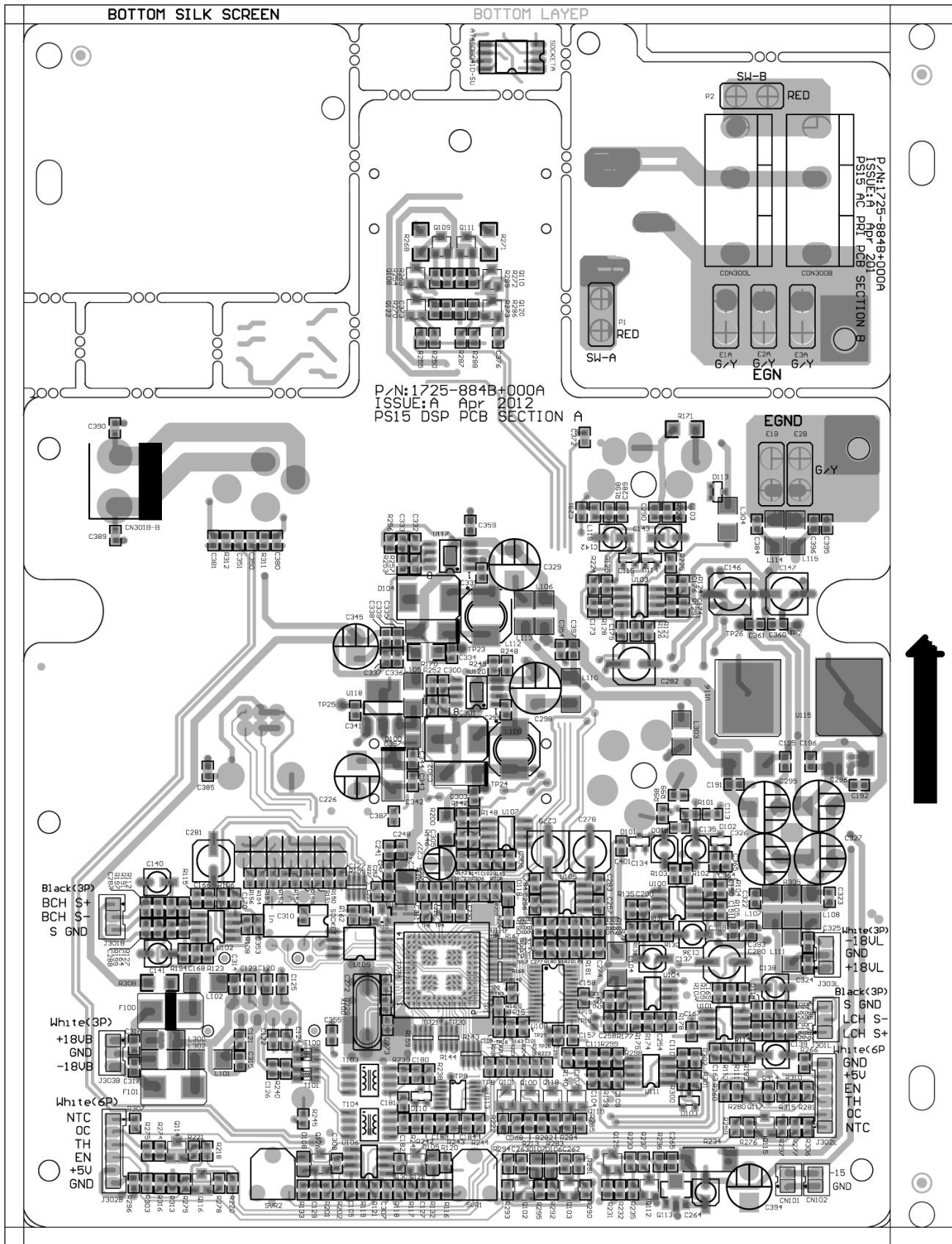
DSP and AC Inlet PCB Bottom Silk and Etch
