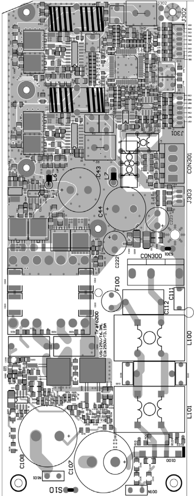
Amplifier/SMPS PCB Topside Etch Layout
