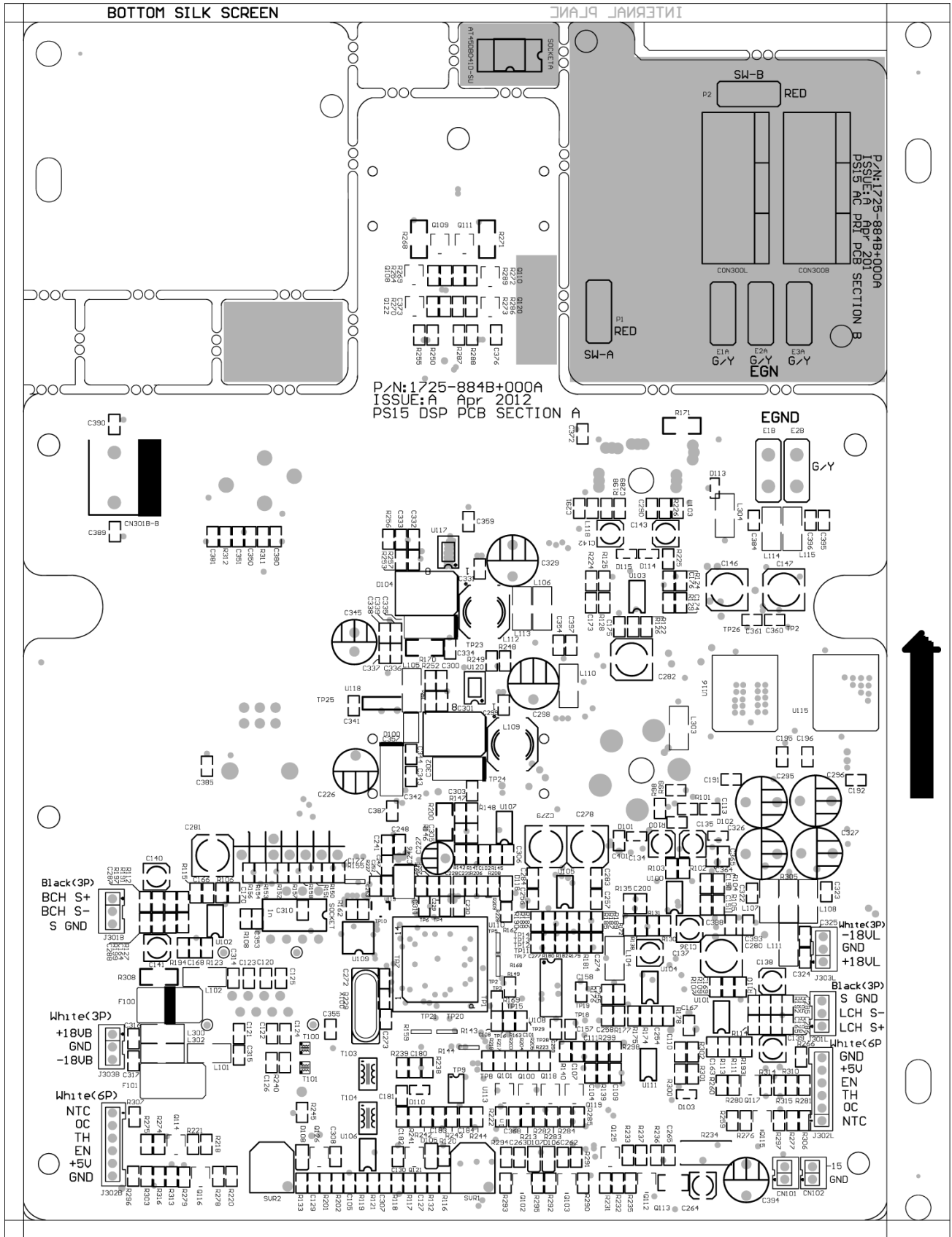
DSP and AC Inlet PCB Bottom Silk and Internal Layer 2
