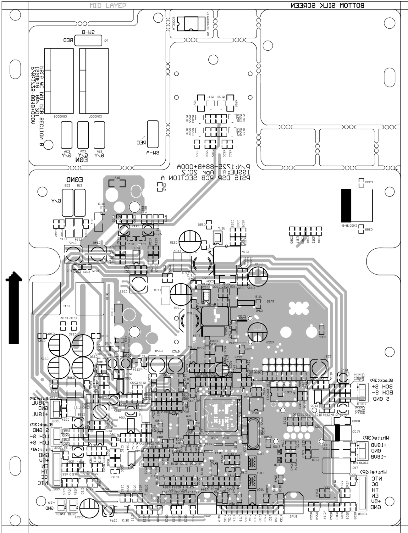
DSP and AC Inlet PCB Bottom Silk and Internal Layer 1
