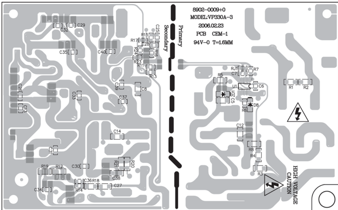
Switch Mode Power Supply PCB Bottom Etch and Component Layout
