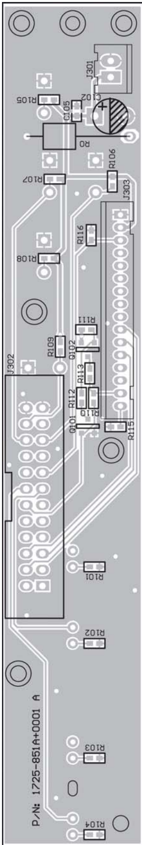
Button and LED PCB Top Etch and Component Layout
