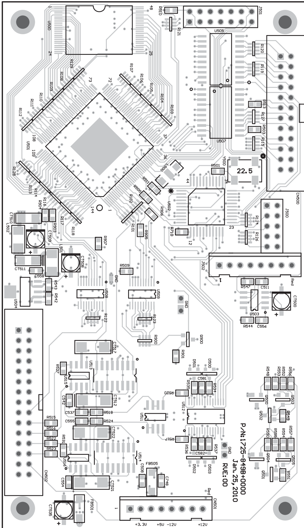
DSP PCB Top Etch Layer and Component Layout
