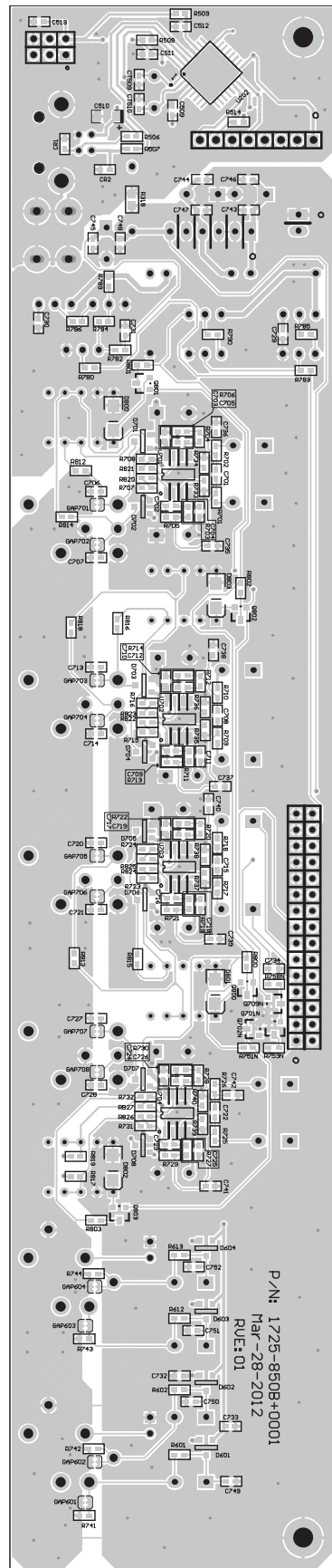
Input/Output PCB Bottom Etch and Component Layout
