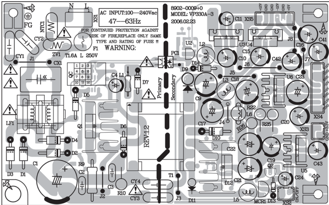
Switch Mode Power Supply PCB Top Etch and Component Layout
