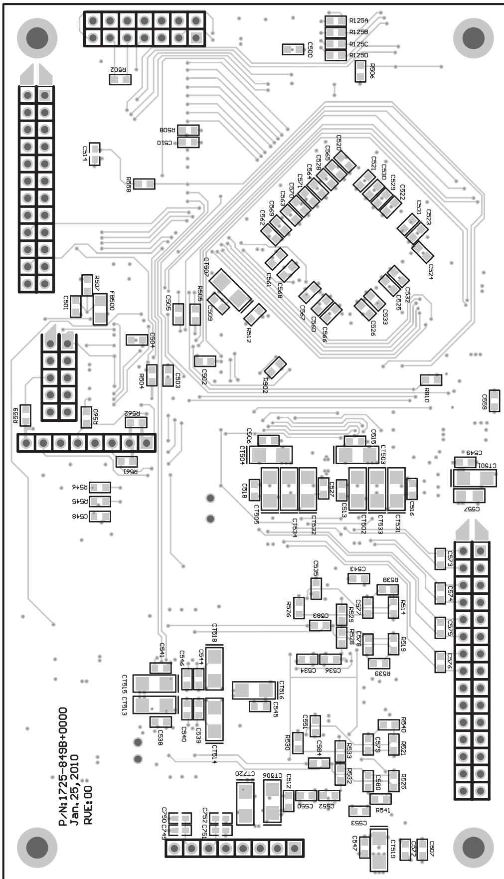
DSP PCB Bottom Etch Layer and Component Layout
