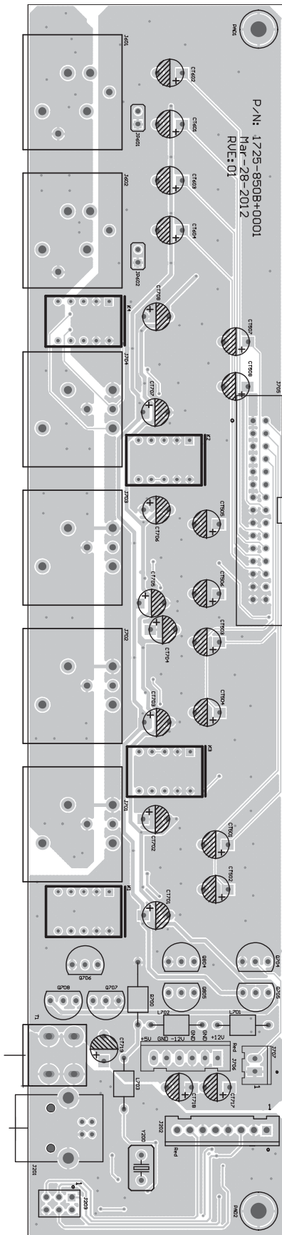
Input/Output PCB Top Etch and Component Layout
