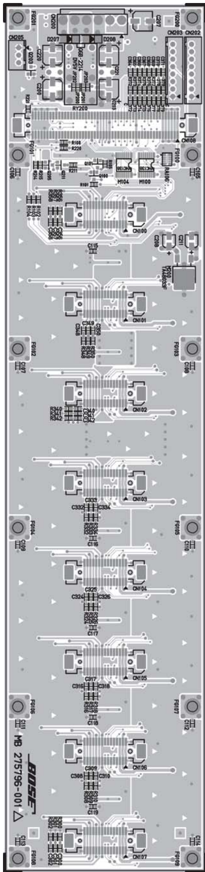
Figure 8. Motherboard Top Etch Layout Diagram
