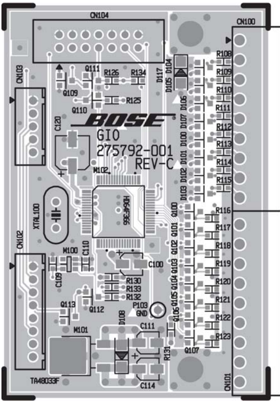
Figure 20. GPIO PCB Topside Etch Layout Diagram
