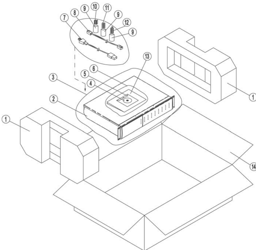
Figure 1. ESP-88 Chassis Packing View
