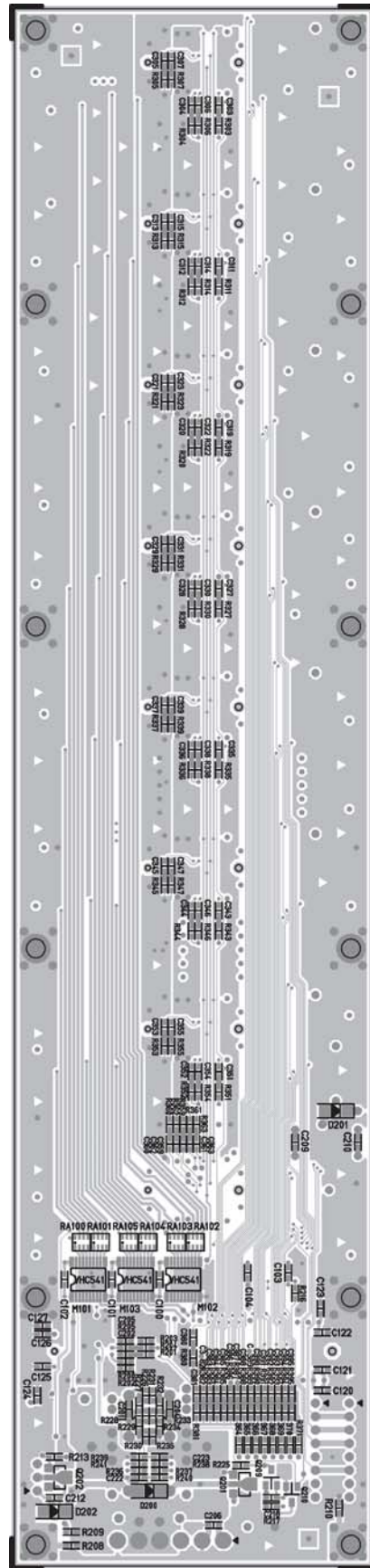
Figure 11. Motherboard Bottom Etch Layout Diagram
