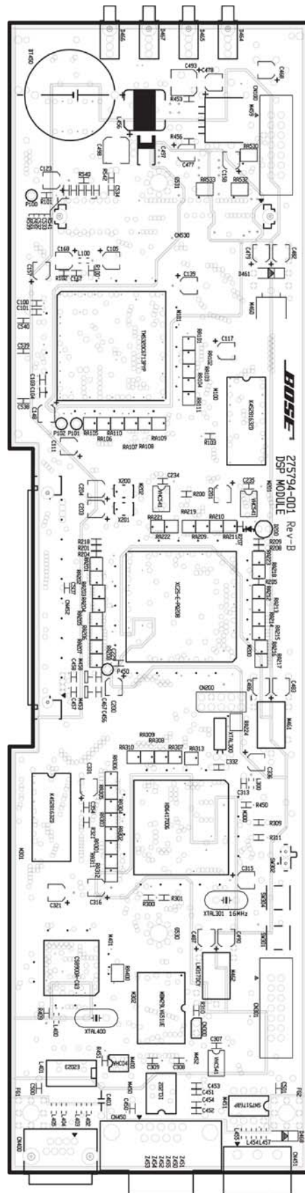
Figure 17. DSP PCB VCC Etch Layout Diagram
