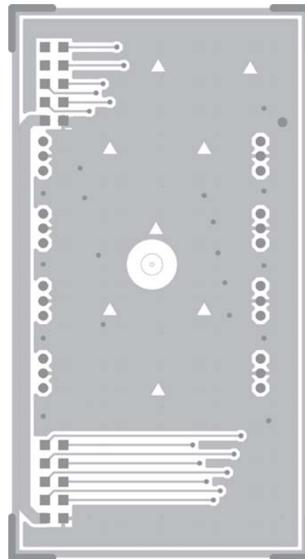
Figure 27. LED PCB Bottom Etch Layout Diagram
