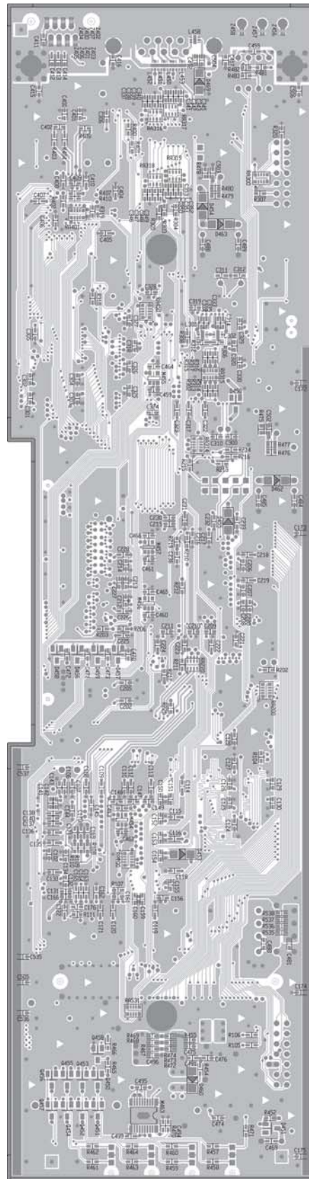
Figure 19. DSP PCB Bottom Etch Layout Diagram
