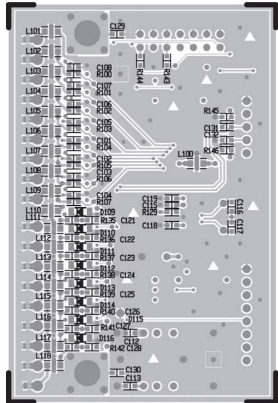
Figure 23. GPIO PCB Bottom Etch Layout Diagram
