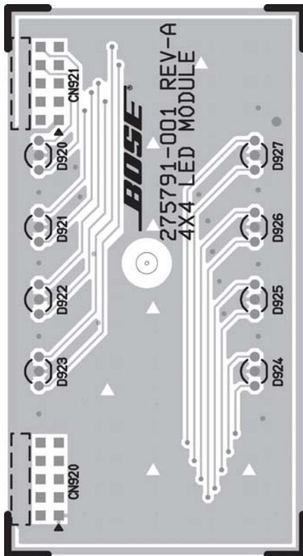
Figure 26. LED PCB Topside Etch Layout Diagram
