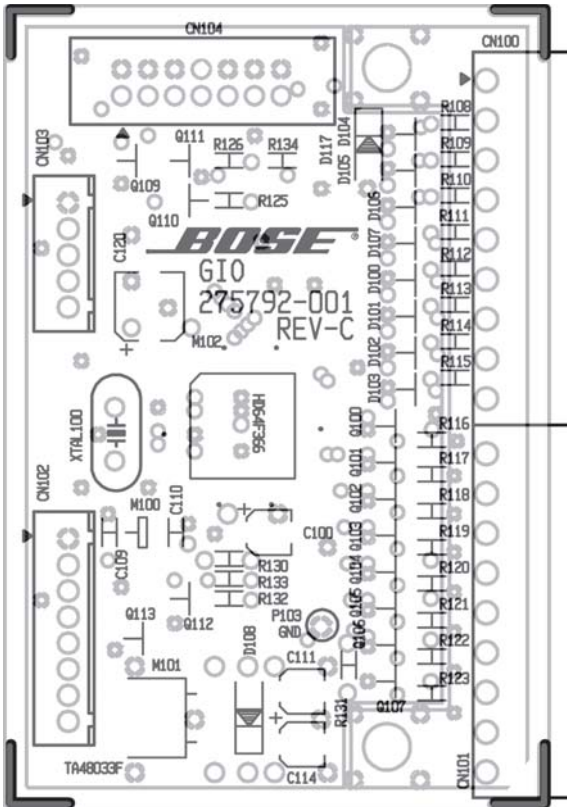
Figure 22. GPIO PCB GND Etch Layout Diagram
