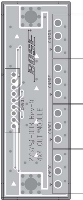
Figure 24. Output PCB Topside Etch Layout Diagram
