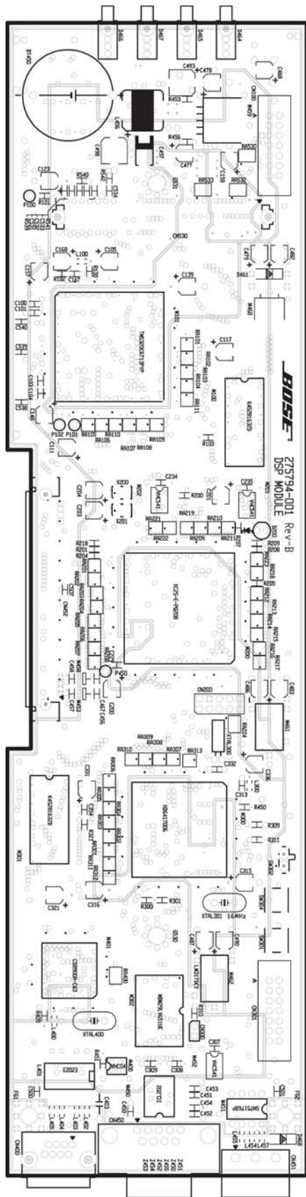
Figure 18. DSP PCB GND Etch Layout Diagram
