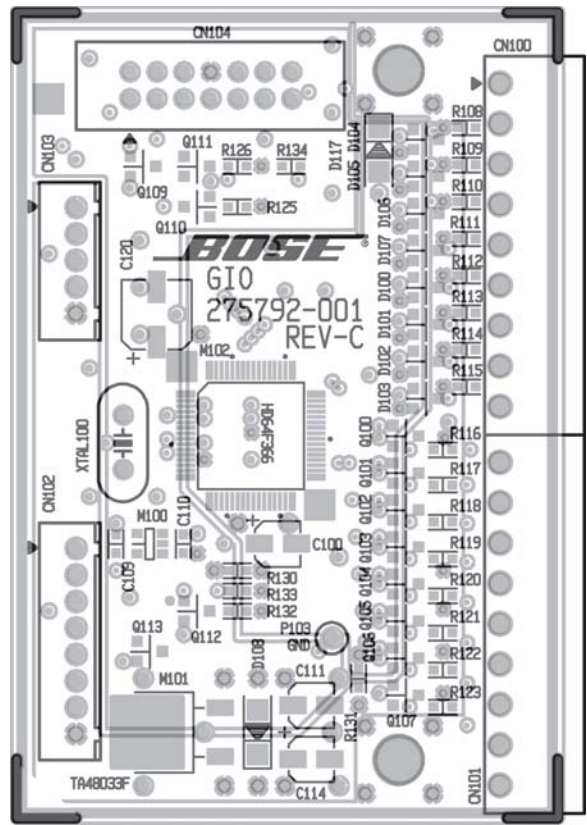
Figure 21. GPIO PCB VCC Etch Layout Diagram
