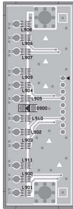
Figure 25. Output PCB Bottom Etch Layout Diagram
