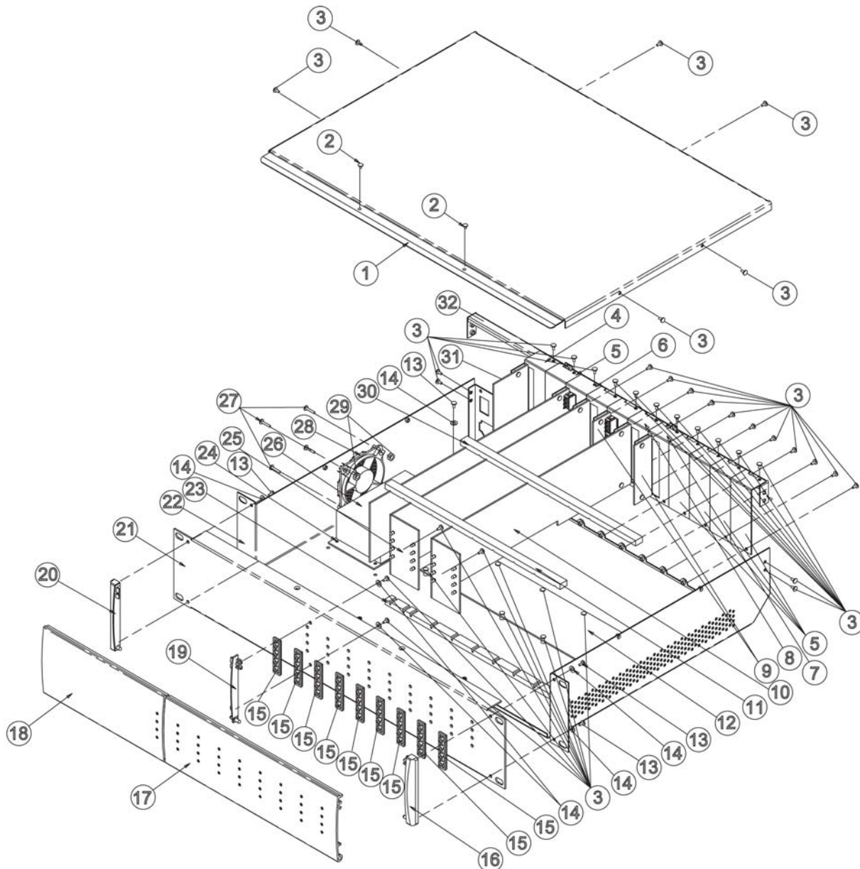
Figure 4. ControlSpace ESP-88 Chassis Exploded View
