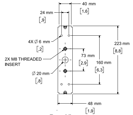
Rear View BRACKET ONLY
