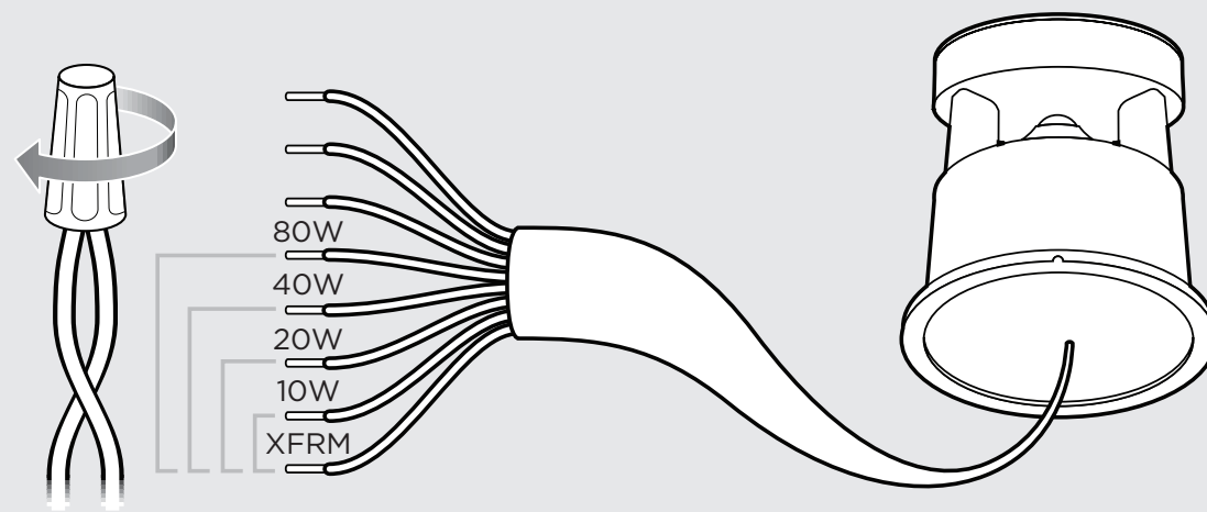
XFRM + 80W OR 40W OR 20W OR 10W
