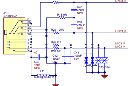
ANALOG INPUT#1
