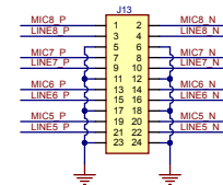
ANALOG INPUT INTERFACE TO MAIN PCB
