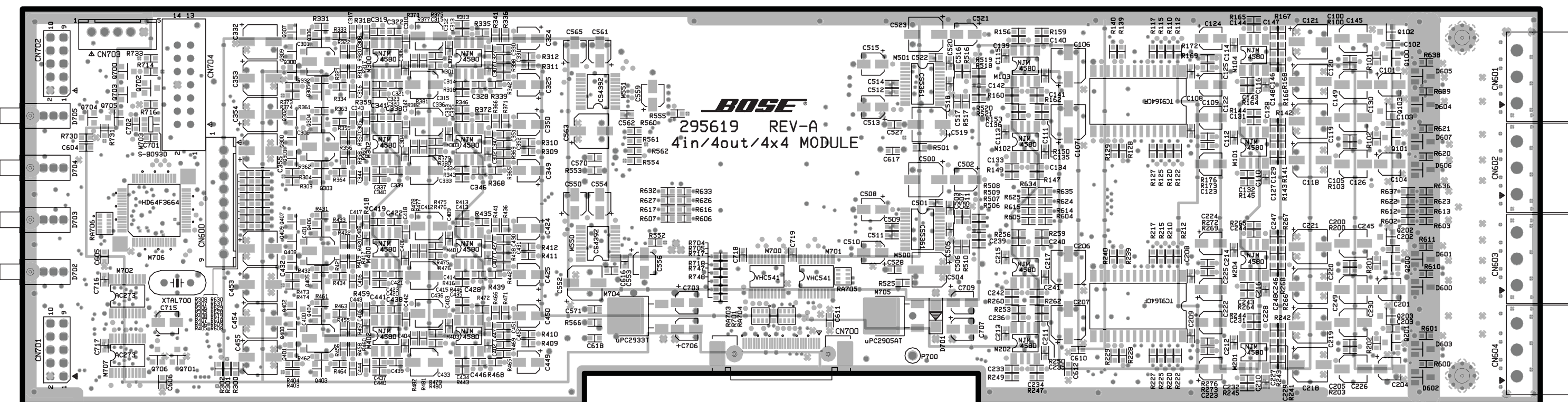
4x4 Series II MIC/Line Input PCB L2 VCC Etch Layout Diagram ControlSpace® ESP-88C and ESP-00 Chassis
