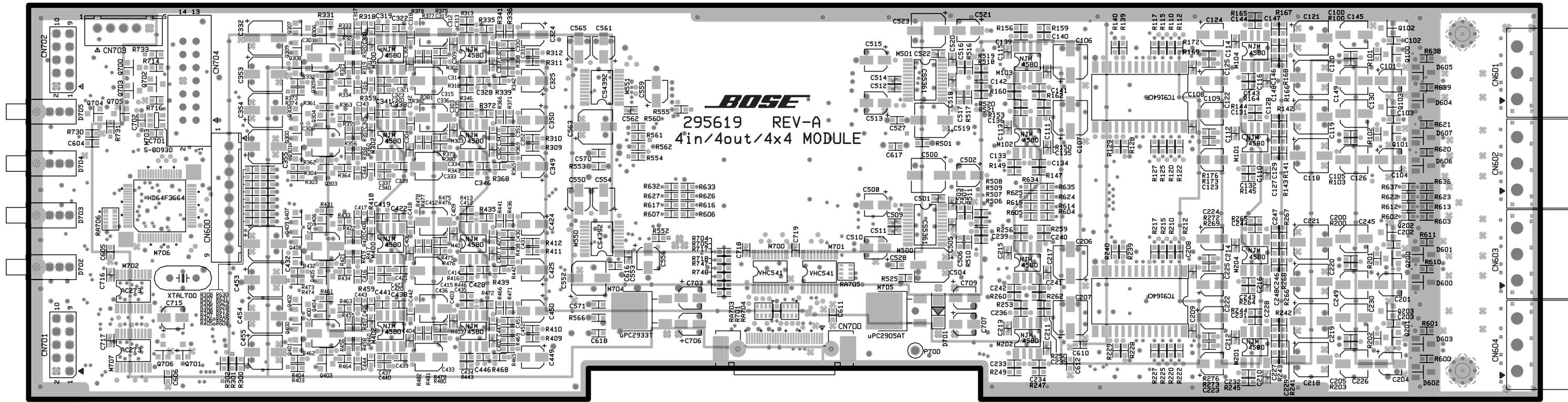
4x4 Series II MIC/Line Input PCB L3 GND Etch Layout Diagram
