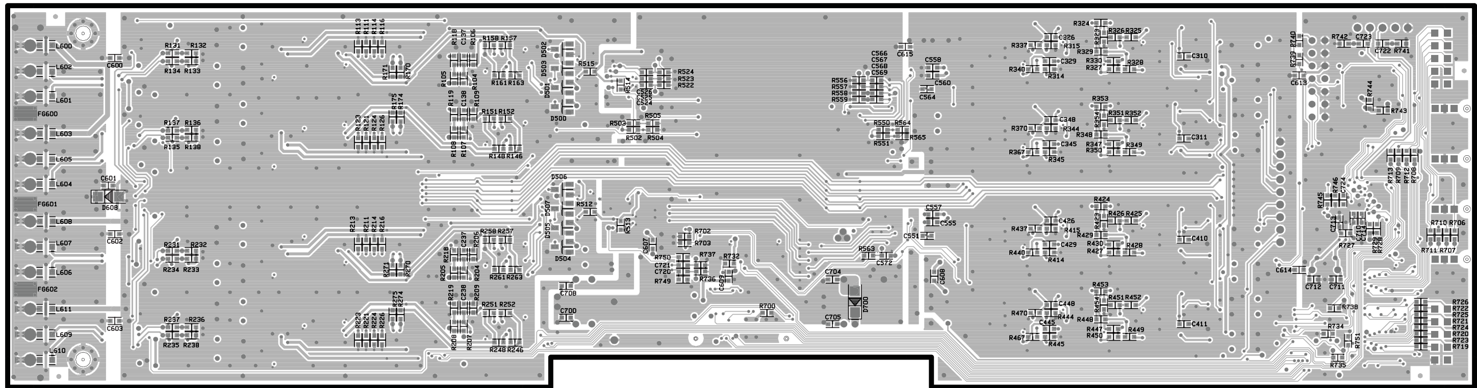
4x4 Series II MIC/Line Input PCB L4 Bottom Etch Layout Diagram ControlSpace® ESP-88C and ESP-00 Chassis
