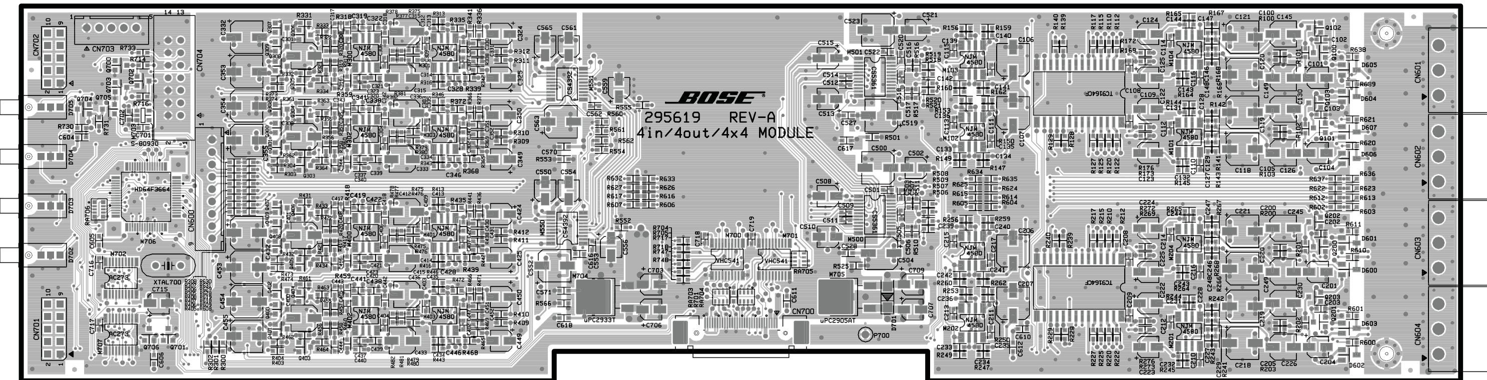
4x4 Series II MIC/Line Input PCB L1 Topside Etch Layout Diagram
